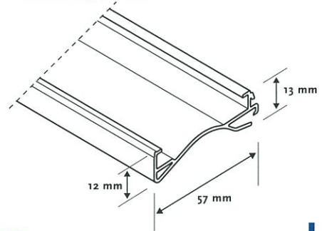
Back/Top profile
